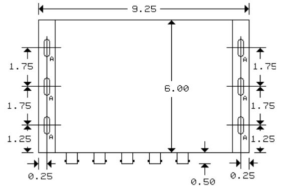
A = 0.20 x 0.70 OVAL CUTOUT
