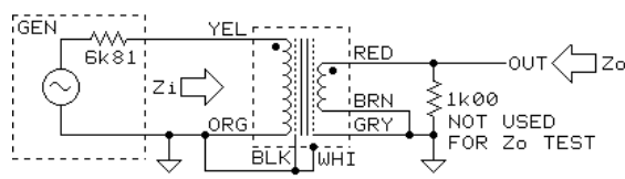
TEST CIRCUIT 1
