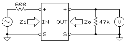
TEST CIRCUIT 1
