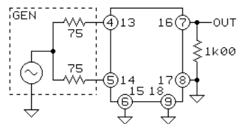
TEST CIRCUIT 2
