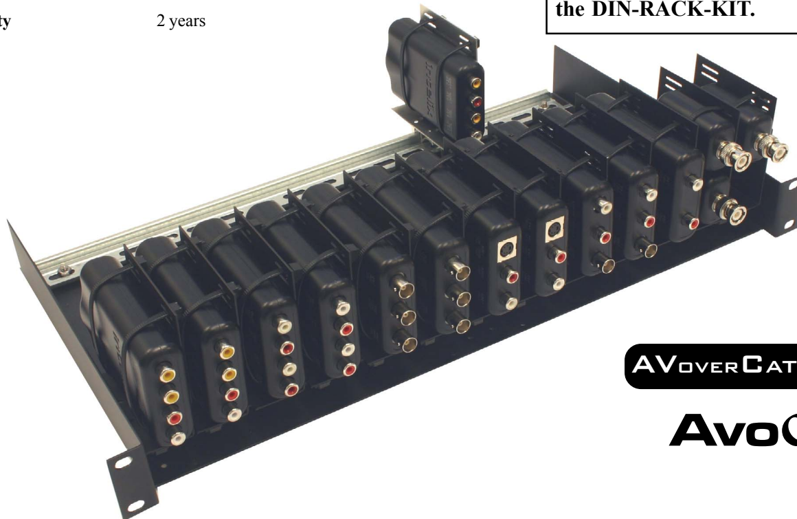
Up to 26 Intelix AVO-CLIPs mount to the DIN-RACK-KIT.
