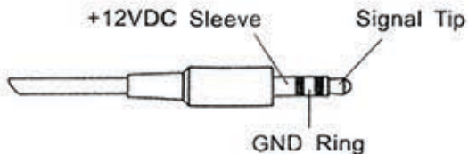
Conductors on 1/8" (3.5mm) stereo mini-plug
